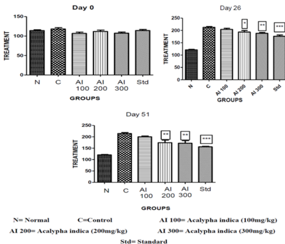
Fig 1: Effect of Ethanol and the Administration of A. indica on SGOT
